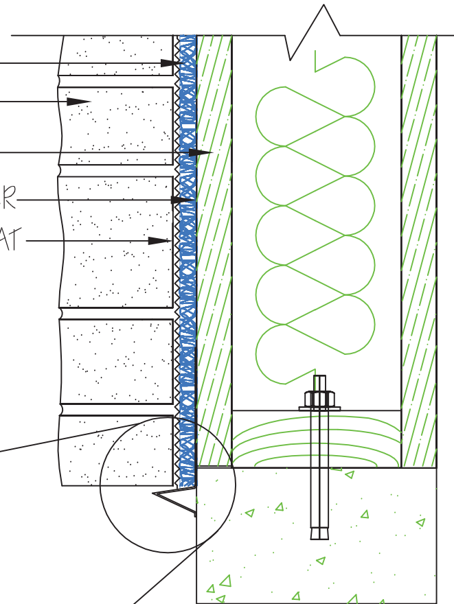
STONE VENEER DETAIL @ BOTTOM OF WALL, WEEP SCREED
