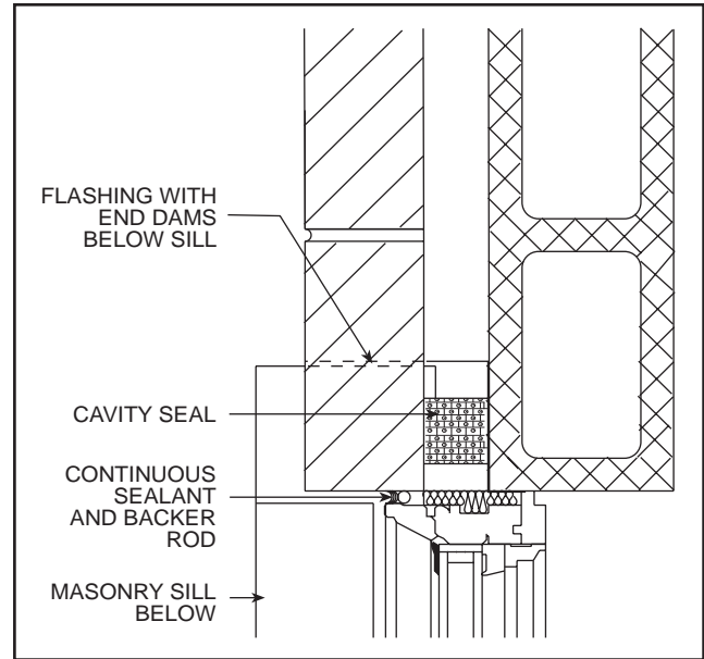
Window Jamb Detail with Cavity Seal FIG. 10
