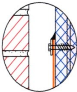
FLASHING SECURED WITH A TERMINATION BAR
