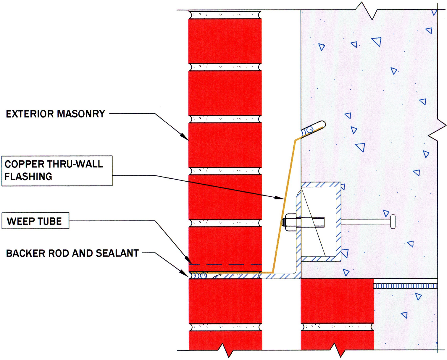
COPPER FLASHING DETAIL
