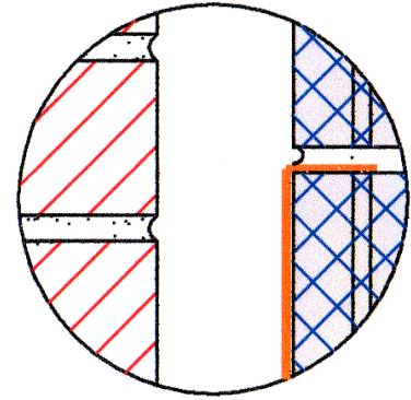
FLASHING SECURED IN A MASONRY JOINT
