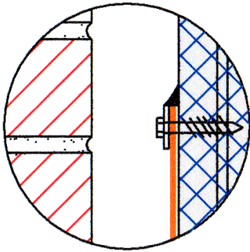
FLASHING SECURED WITH A TERMINATION BAR
