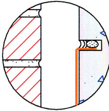
FLASHING SECURED IN A MASONRY REGLET
