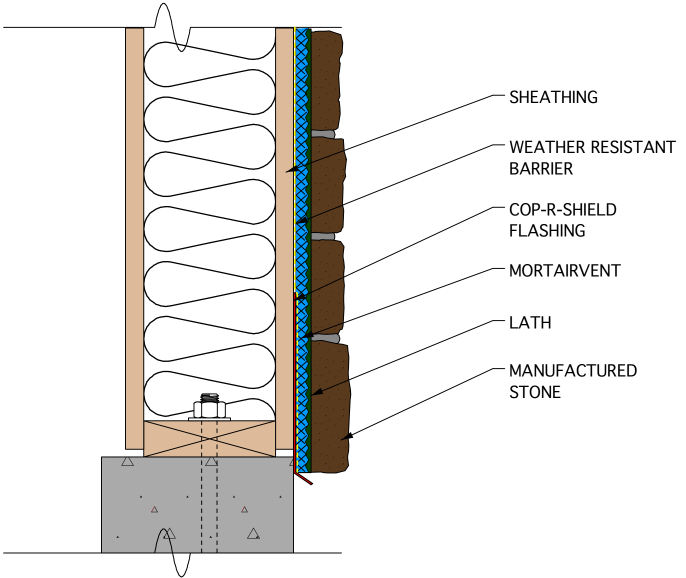
SHEATHING AND WOOD STUD FOUNDATION WALL
