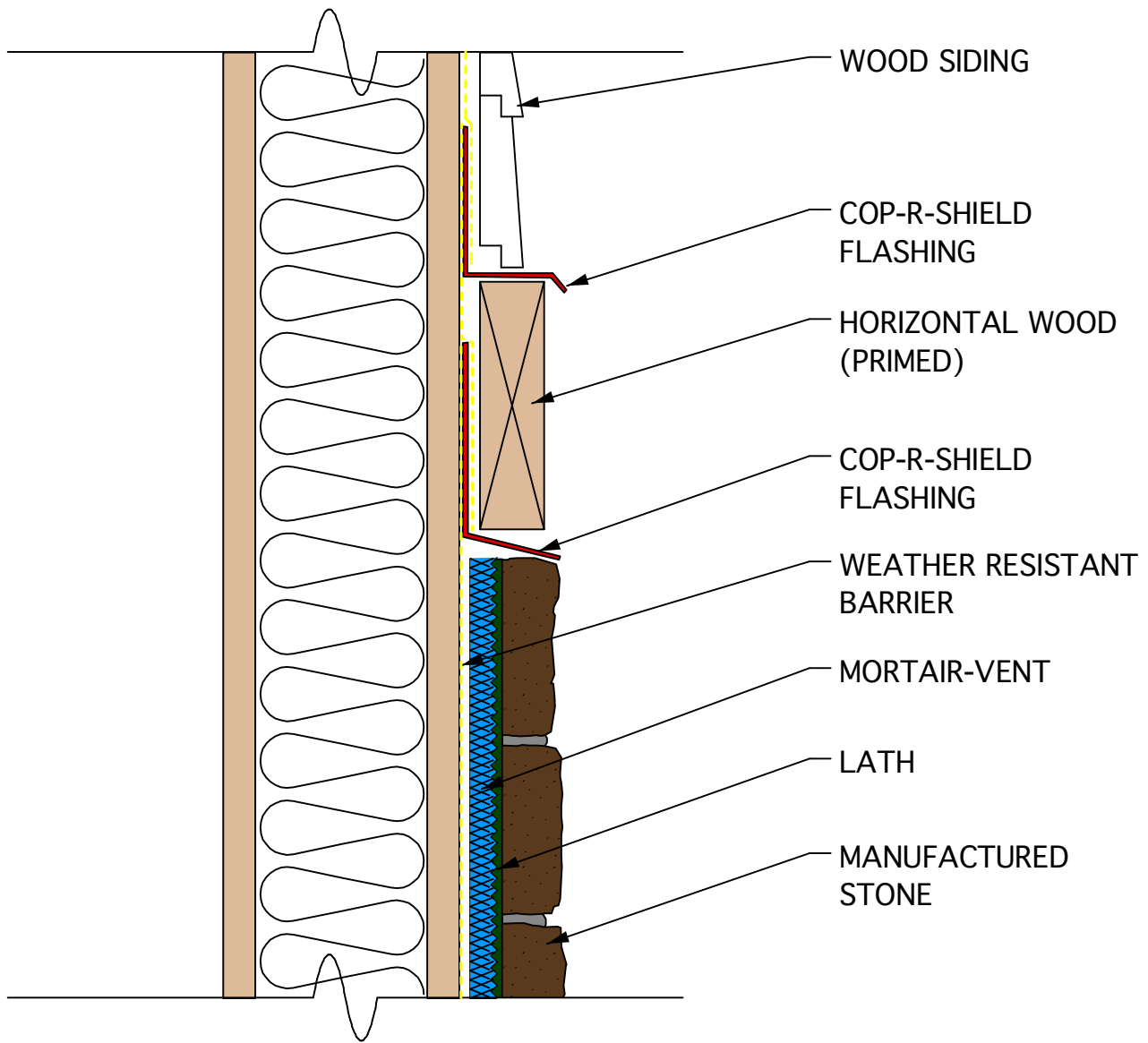
SHEATHING WOOD STUDS HORIZONTAL BASE FLASHING
