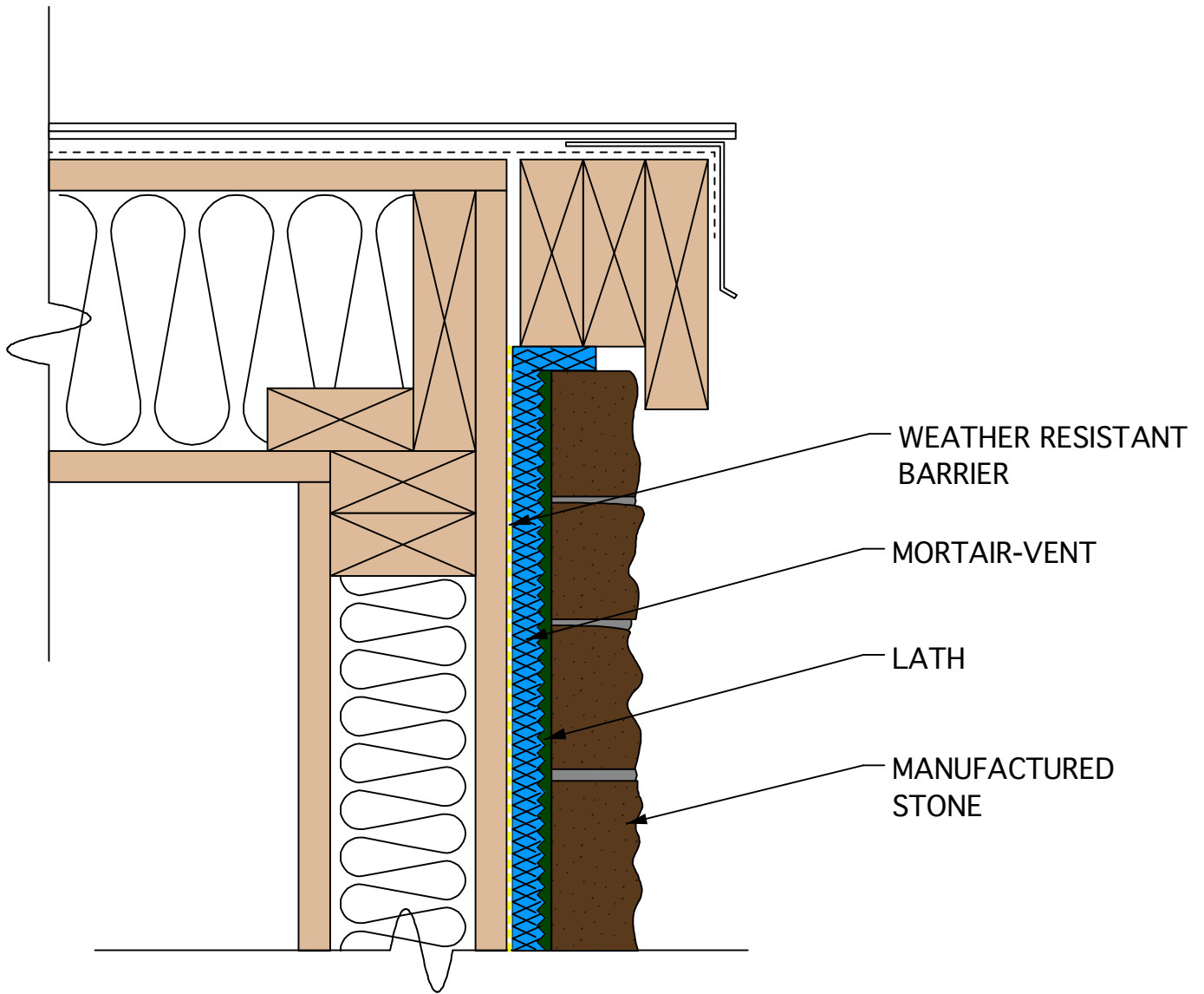
TOP OF FRAMED WALL AT ROOF
