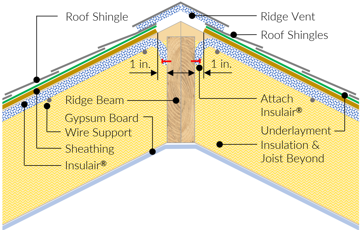
Detail D Ridge Vent/Ridge Beam
