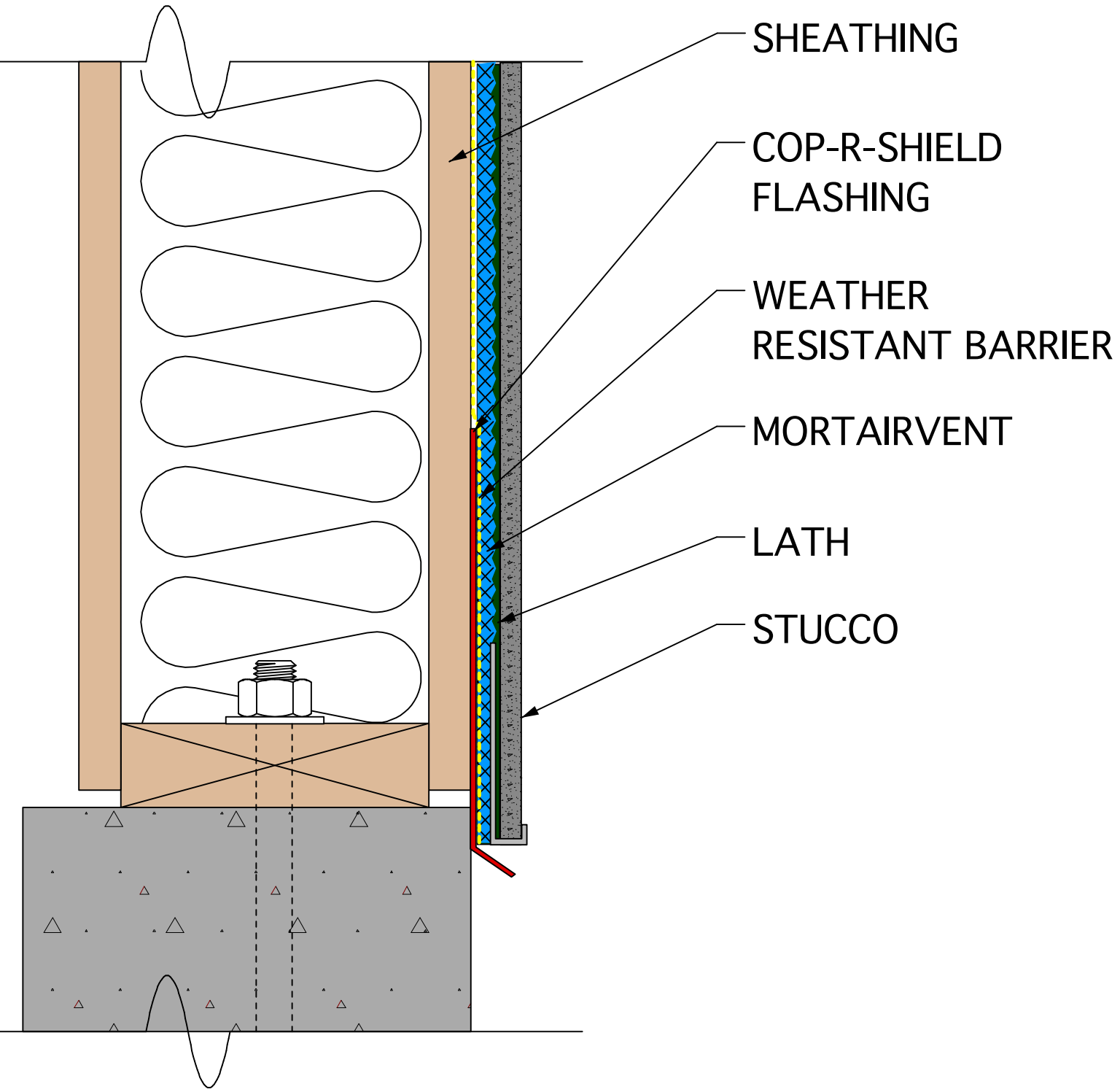
SHEATHING AND WOOD STUD FOUNDATION WALL
